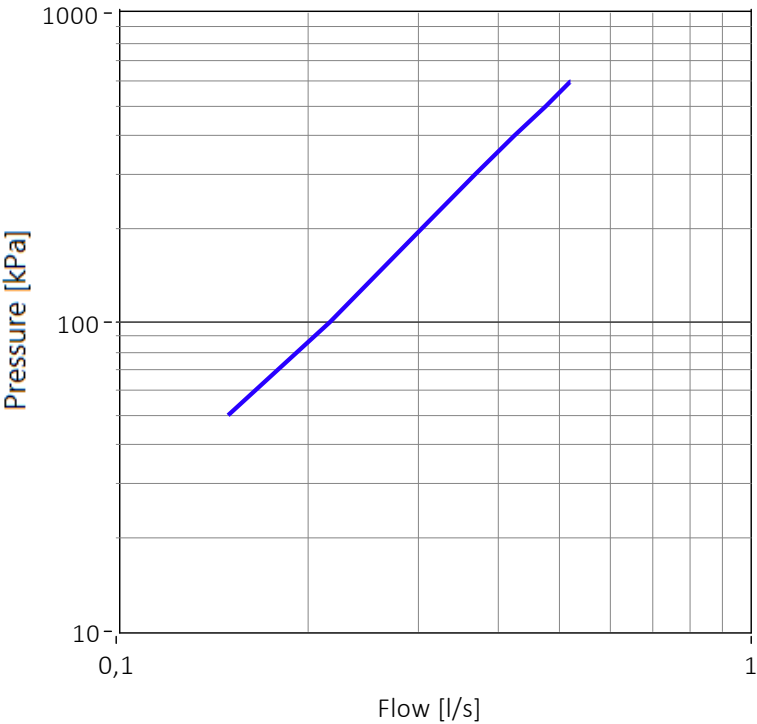
FLOW CHART AS A FUNCTION OF INLET PRESSURE
